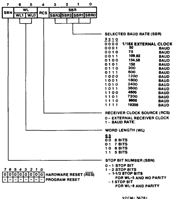
Fig. 4 - CDP65C51/51A control register.
