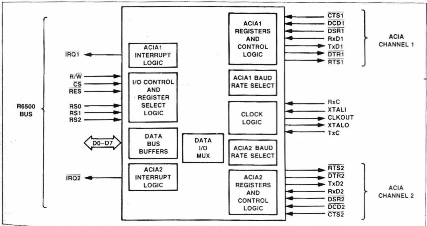
Figure 2. R65C52 DACIA Interface Signals
