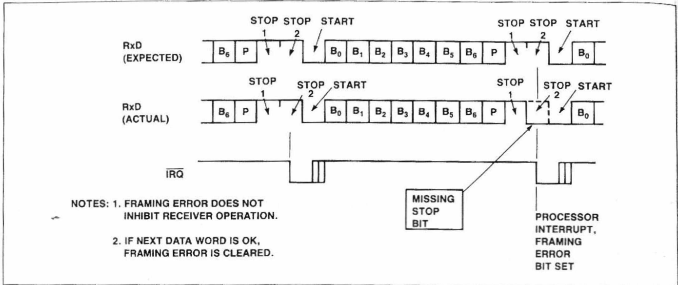
Figure 15. Framing Error
