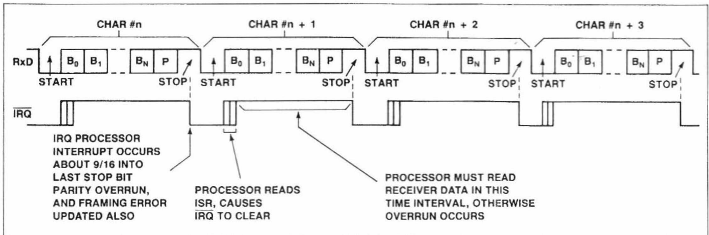
Figure 12. Continuous Data Receive
