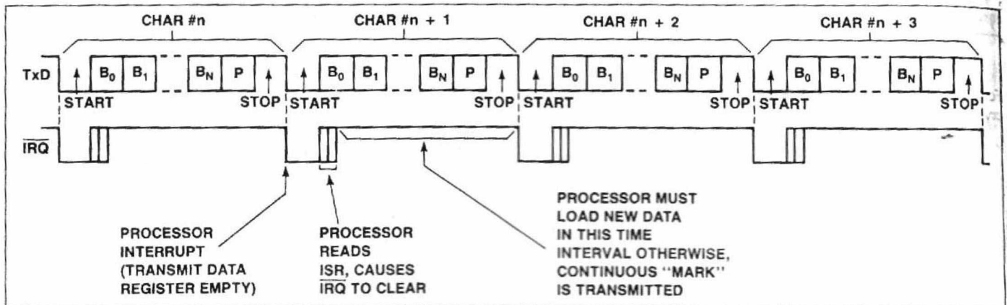
Figure 7. Continuous Data Transmit
