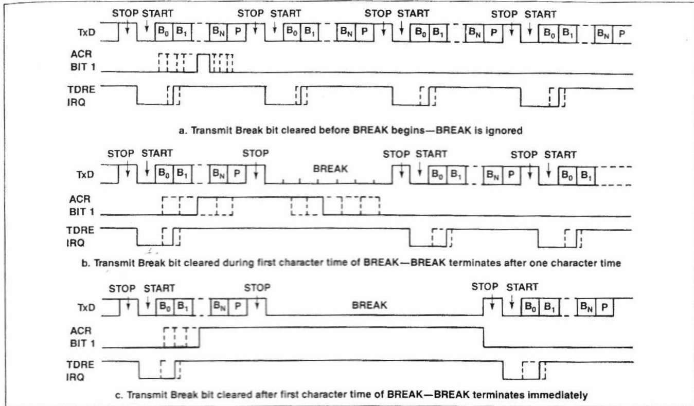
Figure 9. Transmit BREAK
