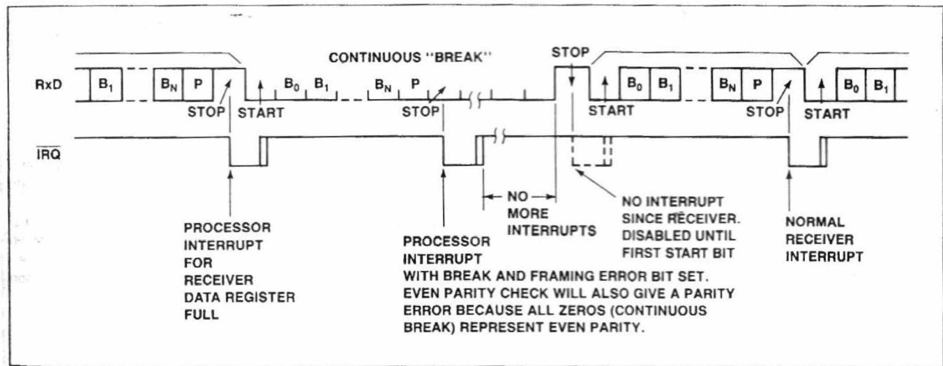
Figure 14. Receive Break Character
