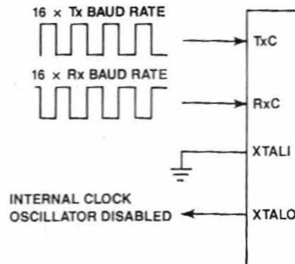
B. Both Channels Use External Clocks
