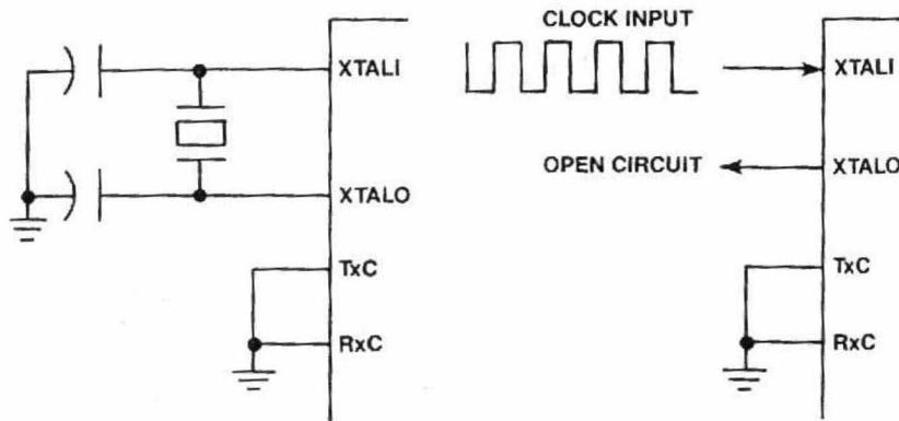
A. Both Channels Use Internal Baud Rate Generator
