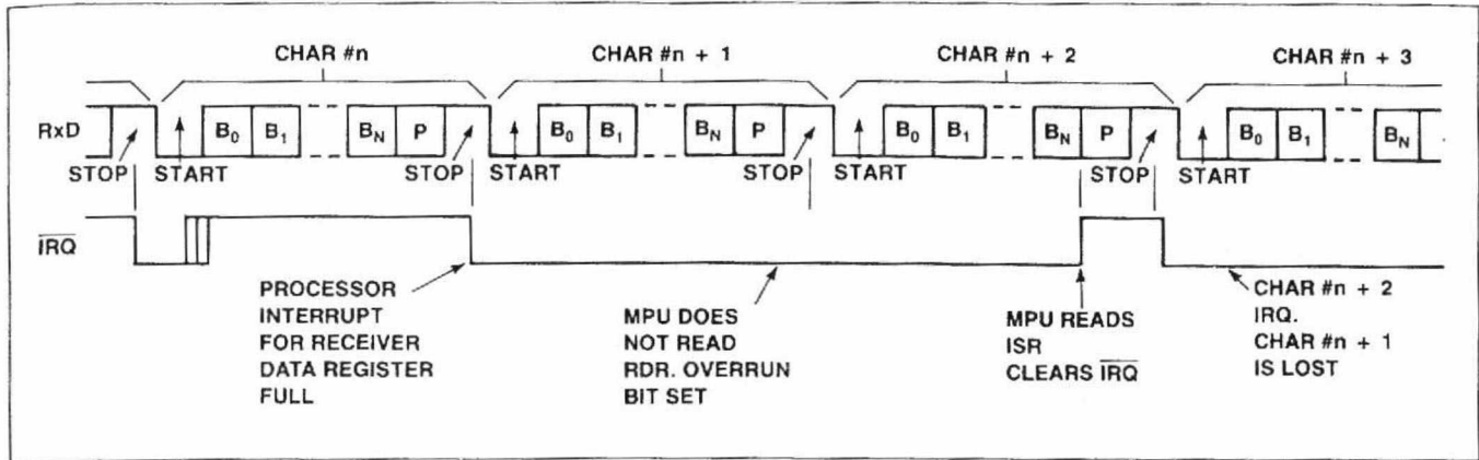
Figure 13. Effects of Overrun on Receiver
