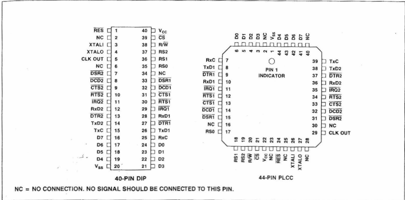
Figure 1. R65C52 Pin Assignments
