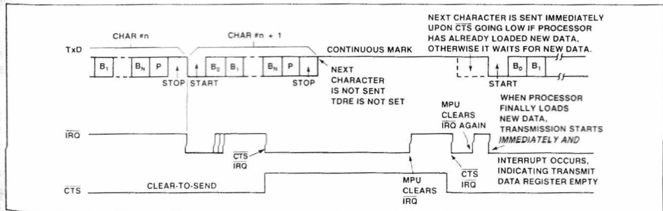
Figure 10. Effects of CTS on Transmitter
